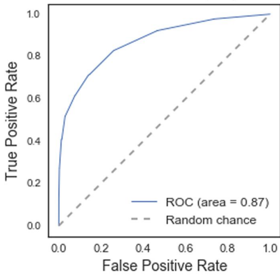
Random Forests ROC (depression)
